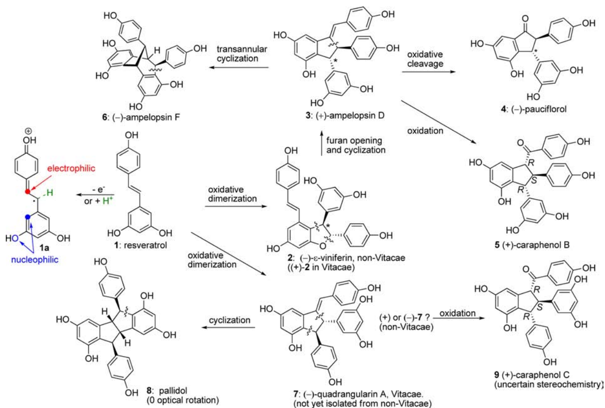
Scheme 1. Some Resveratrol Derived Natural Products 3
