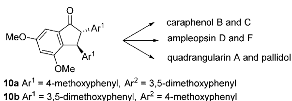
Scheme 2. Use of Indanones in Resveratrol Dimer Synthesis 4,9
